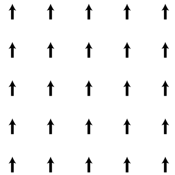
d / The field \hat{y} .
